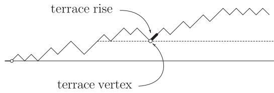
Figure 2. An example of a height 3 terrace showing the terrace rise and terrace vertex.
