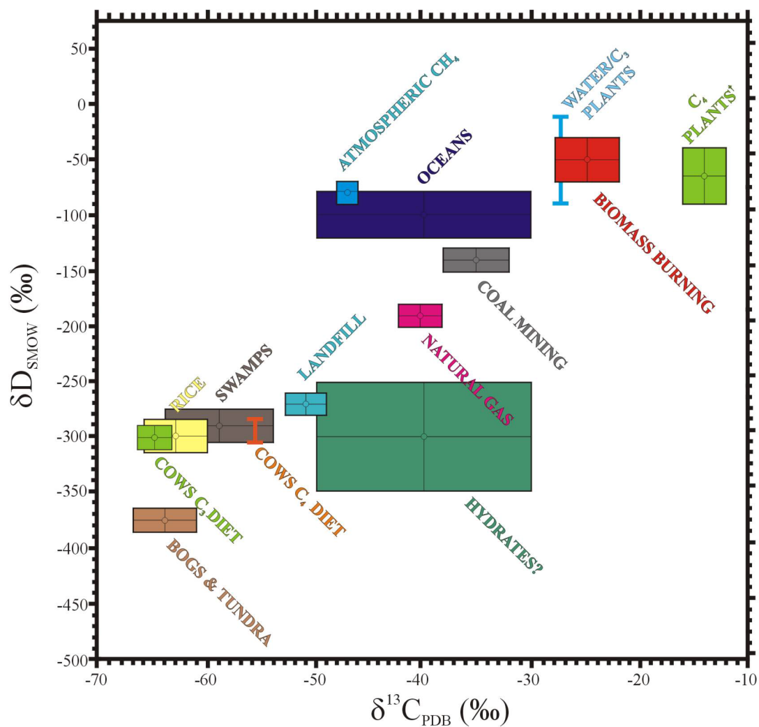
Figure 2.3 - A summary plot of carbon and hydrogen stable isotopic ratios for methane. (Levin et al. , 1993, Levin unpublished data). Range of D/H for C 4 plants from Smith and Zeigler (1990).
